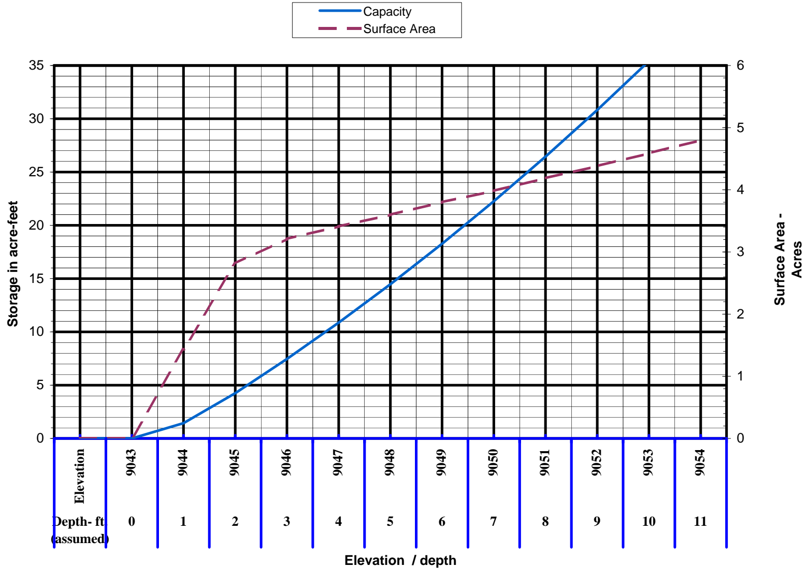
Capacity Table, Lost Park Ranch Reservoir
